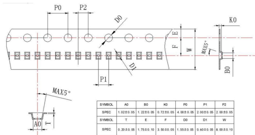
Carrier Tape
