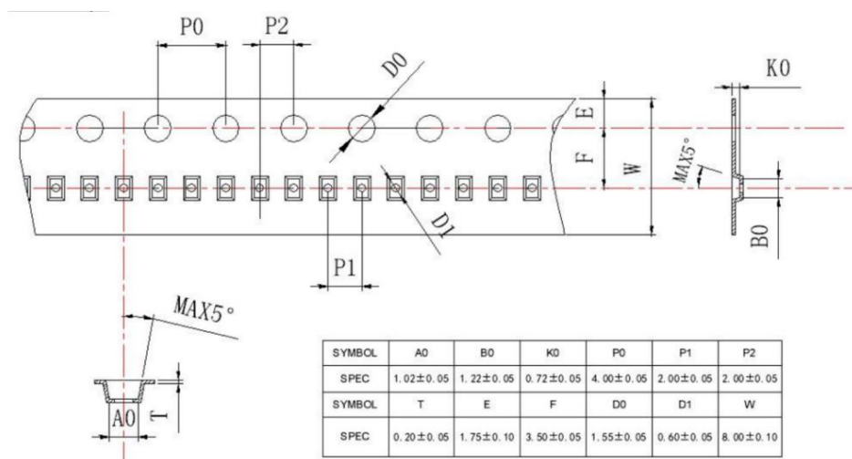
Carrier Tape
