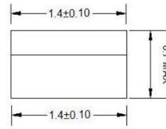
side view(front)
