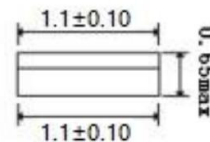
side view(front)
