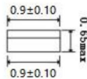
side view(left)
