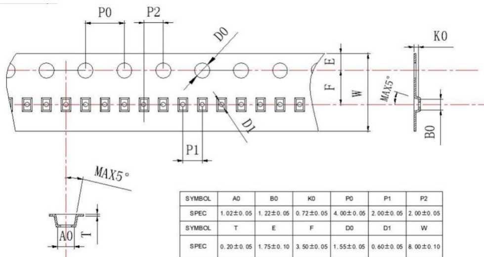
Carrier Tape
