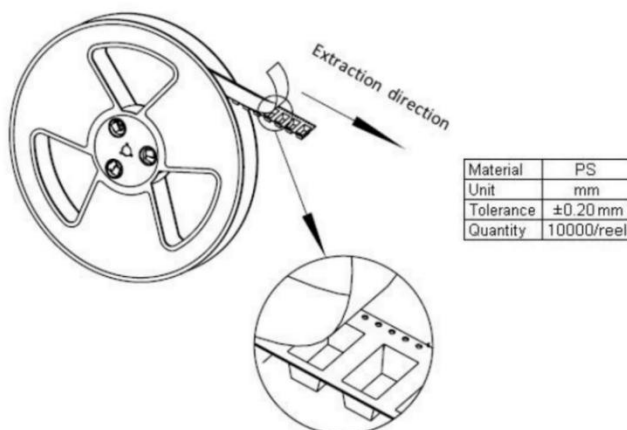
Outer Packing
