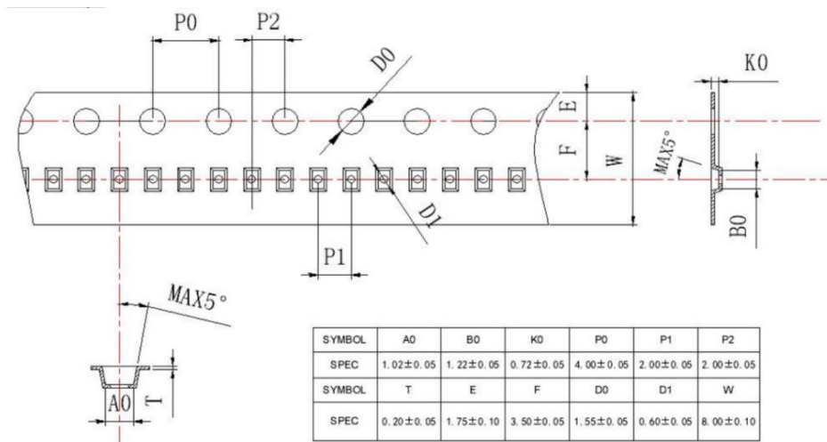
Carrier Tape
