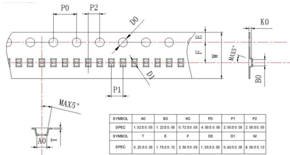
Carrier Tape
