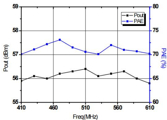
Pout, PAE&Freq.
