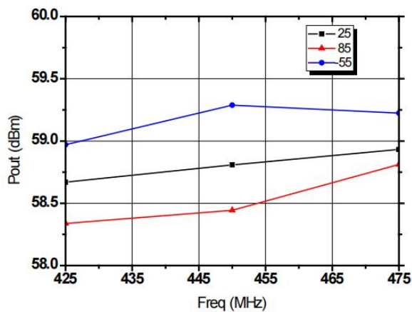
Pout, PAE&Freq.
