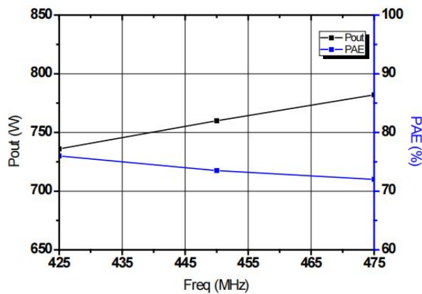
Pout, PAE&Freq.
