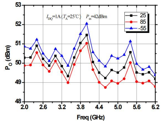
Po&Freq.
