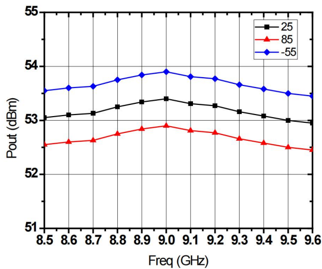
Pout&Freq. @ Different Temp.
