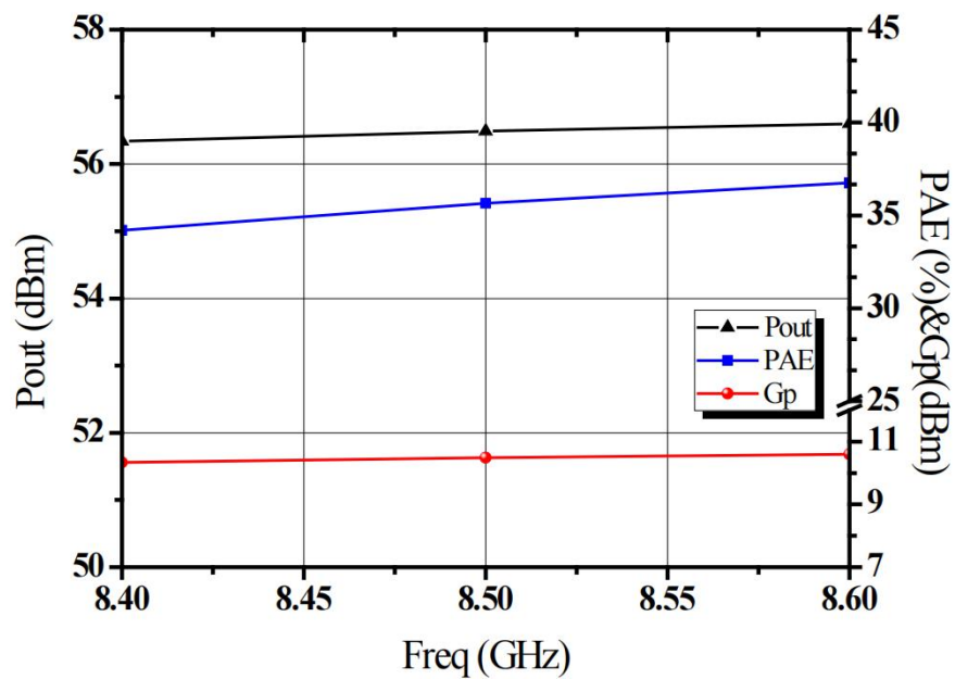
Pout&PAE&Gain VS Freq.
