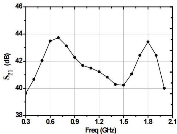
Gain&Freq.
