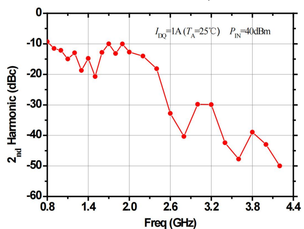
2 nd Harmonic&Freq.
