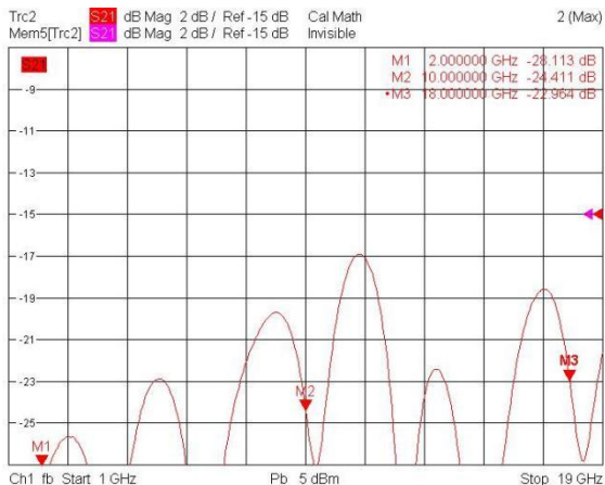
Directivity
