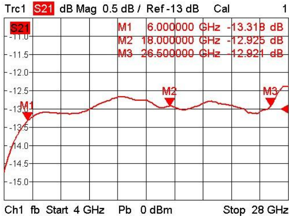
Coupling
