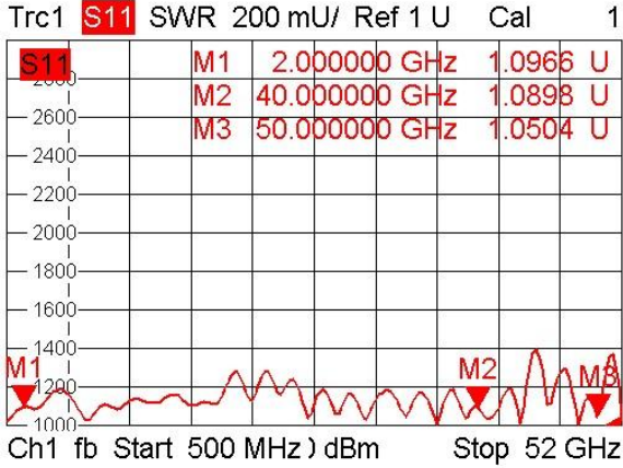
Coupling-Port VSWR
