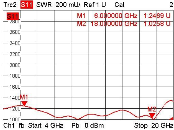
Coupling-Port VSWR
