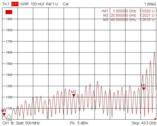
Directivity
