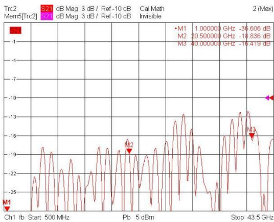
Directivity
