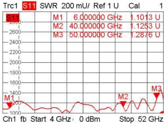
Coupling-Port VSWR
