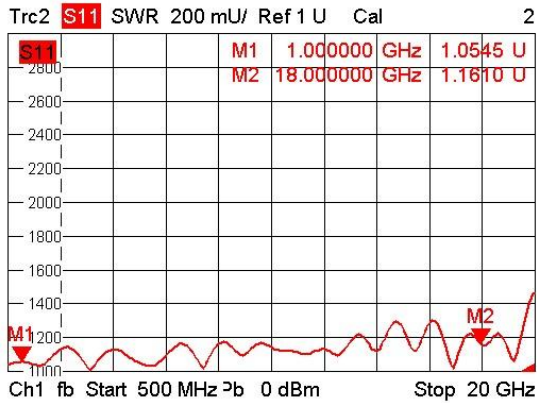
Coupling-Port VSWR
