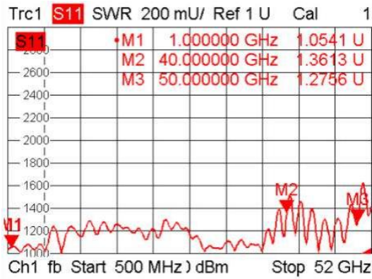
Coupling-Port VSWR
