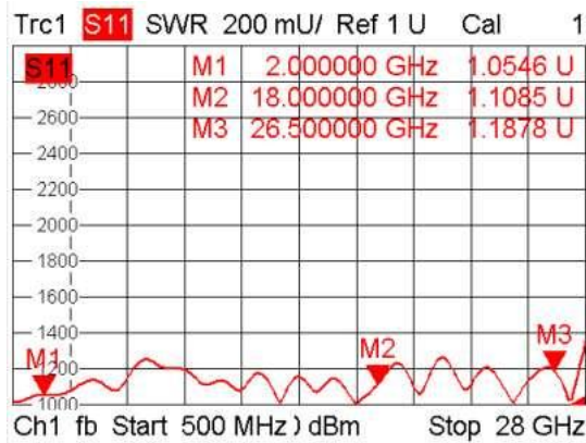
Coupling-Port VSWR
