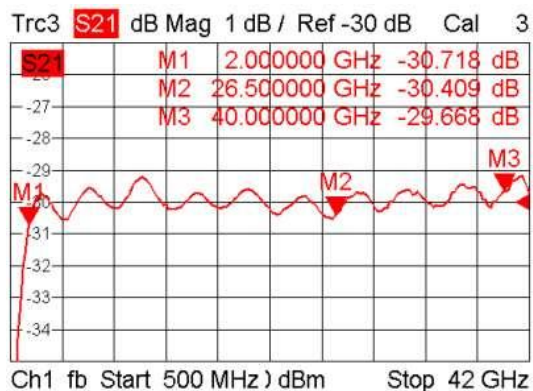
Coupling
