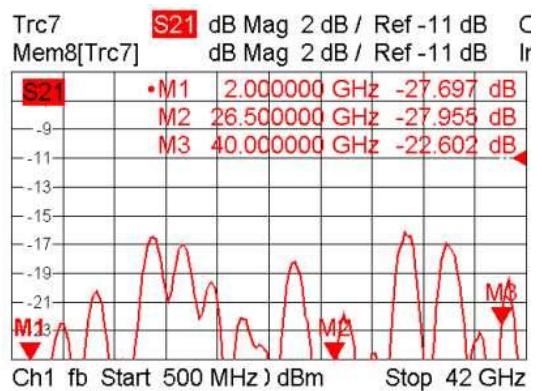
Directivity
