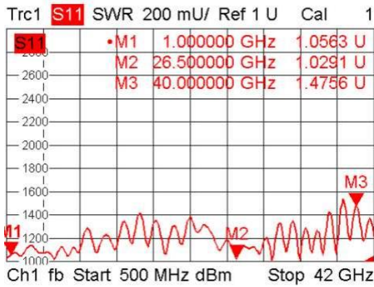
Coupling-Port VSWR
