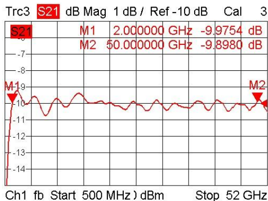
Coupling
