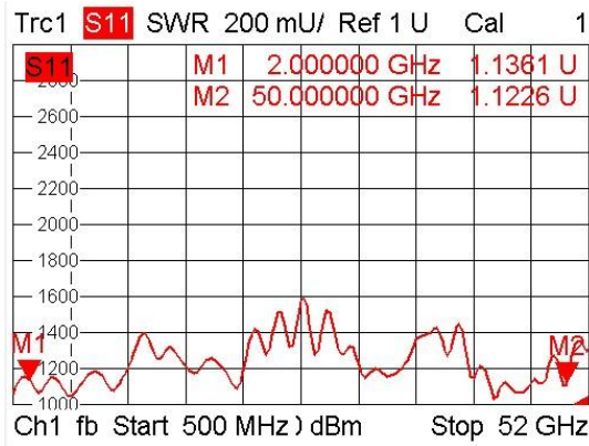
Coupling-Port VSWR
