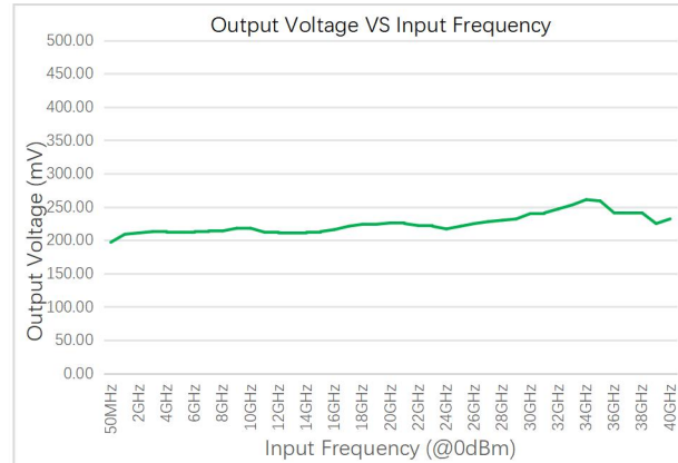
Output Voltage VS Input Frequency
