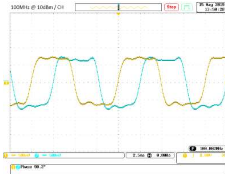
Typical 100MHz waveform, both channels adjusted to 90 degrees offset (500MHz scope).
