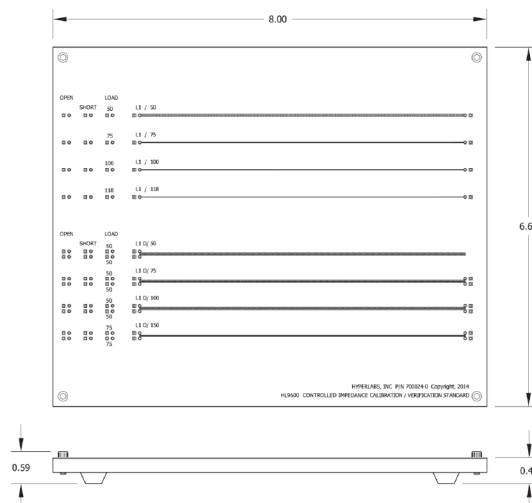
Figure 2: HL9600 dimensional drawing*
